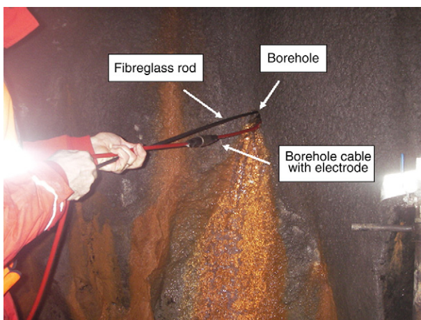
Fig. 8. Photograph of a borehole cable with the thin fibreglass rod.
