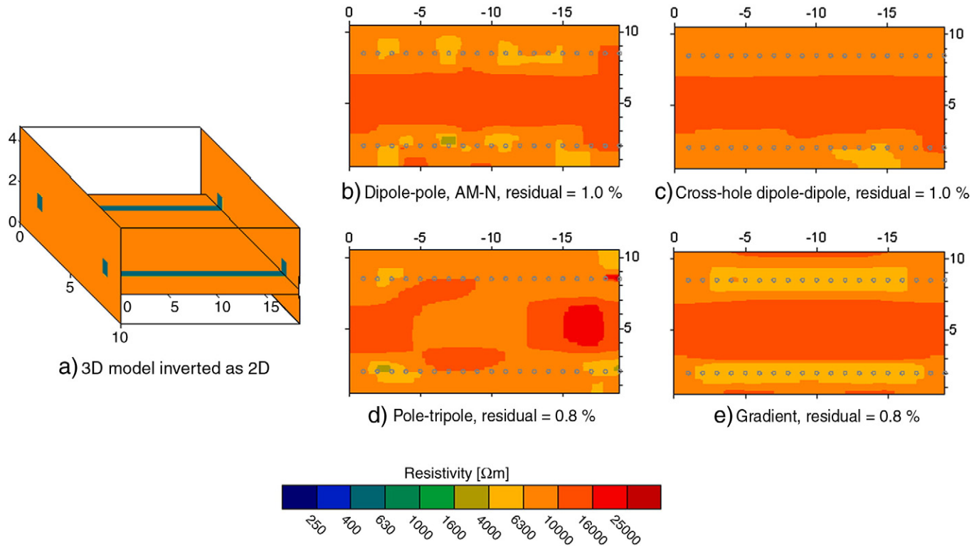
Fig. 3. a) The 3D model is inverted as 2D. The matrix has a resistivity of 8000 \Omega \text{ m} and the borehole has a resistivity of 500 \Omega \text{ m} . Inversion results using b) dipole–pole (AM-N), c) cross-hole dipole–dipole (AM-BN), d) pole–tripole (A-BMN), e) multiple gradient. The distance is in metre.
